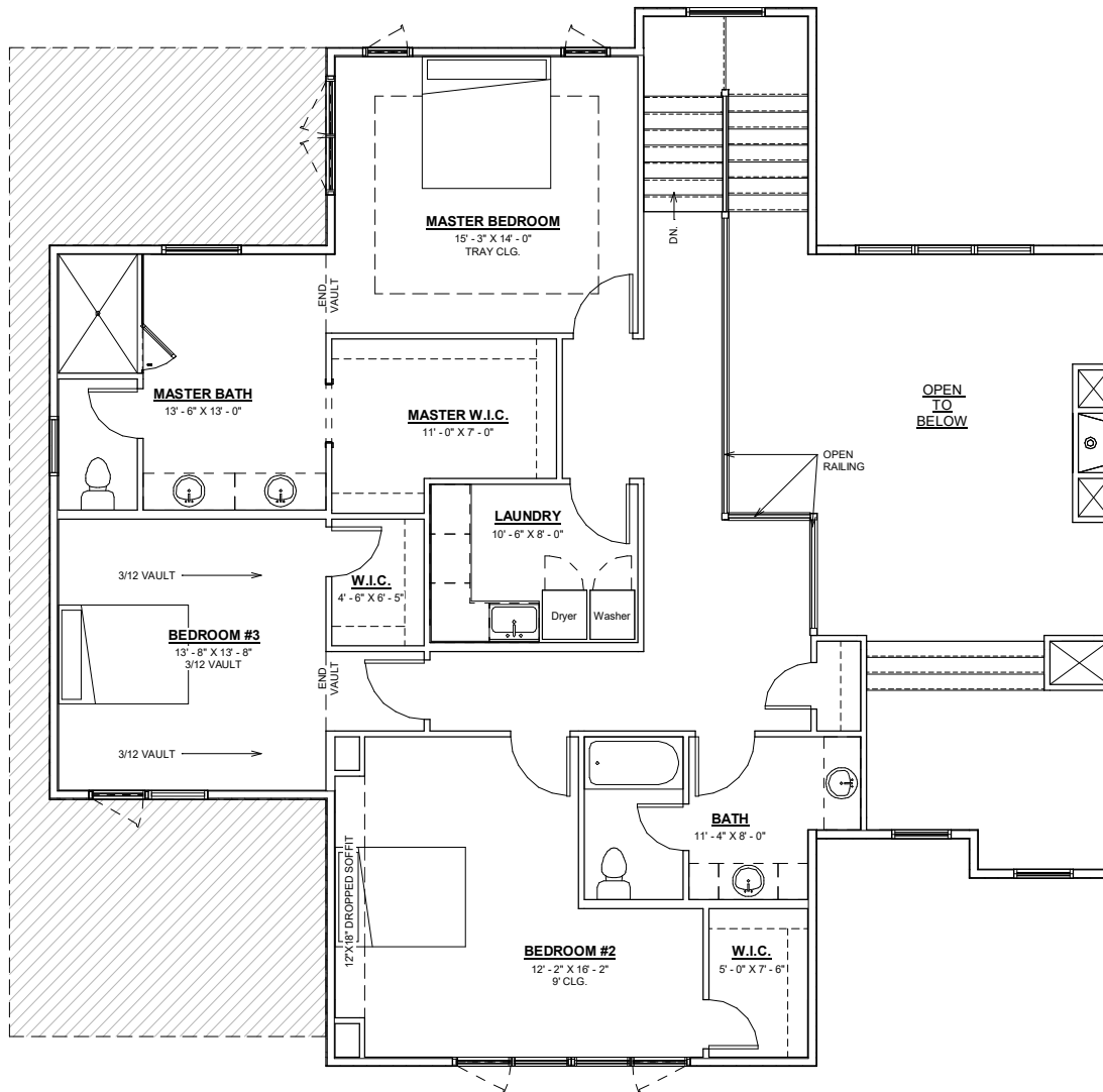
Second Level Floor Plan Second Level Sq. Ft. = 1,612 Sq. Ft.
